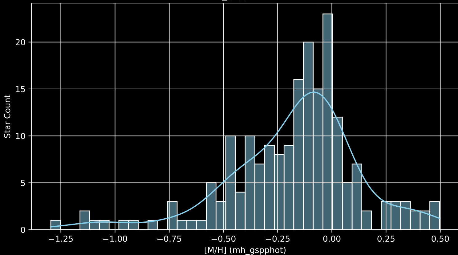
APOGEE DR17 Field: [070-32_MGA [M/H] (mh_gspphot) (n= 195)
