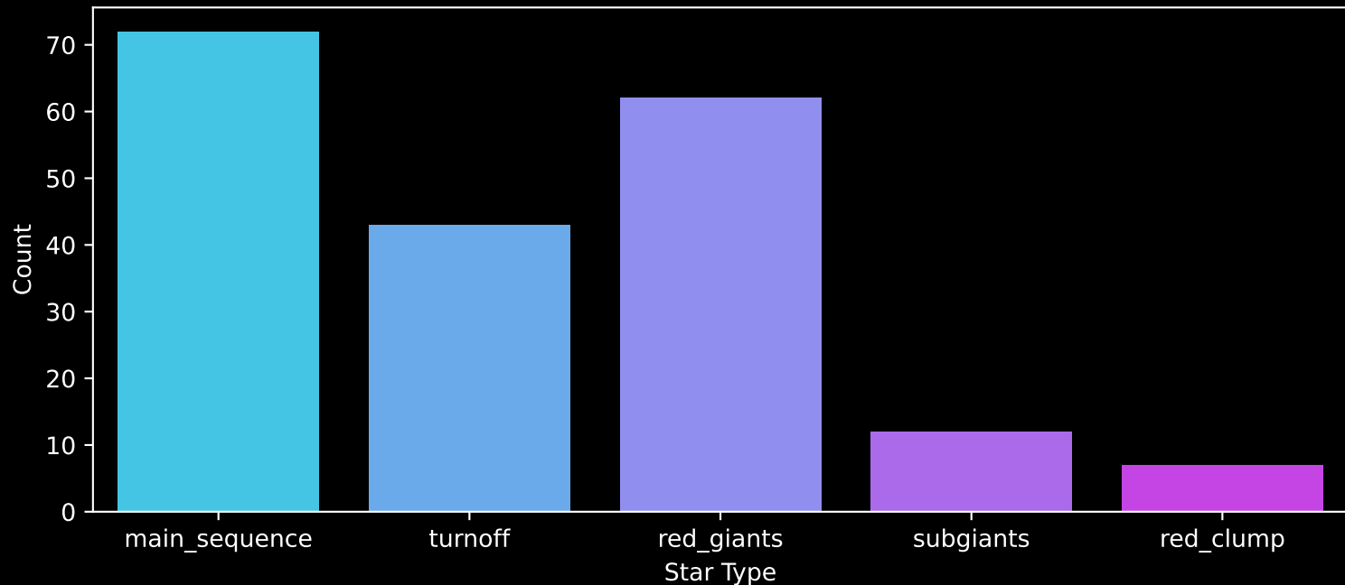
APOGEE DR17 Field: [070-32_MGA] Count plot of Star Type
