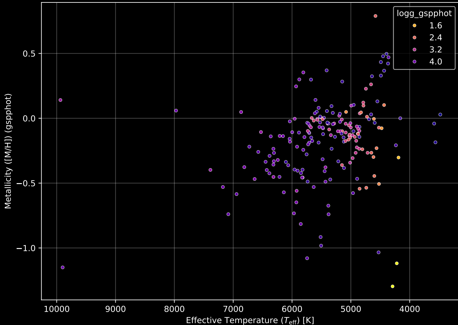
APOGEE DR17 Field: [070-32_MGA] Stellar Population Parameters (n= 196)
