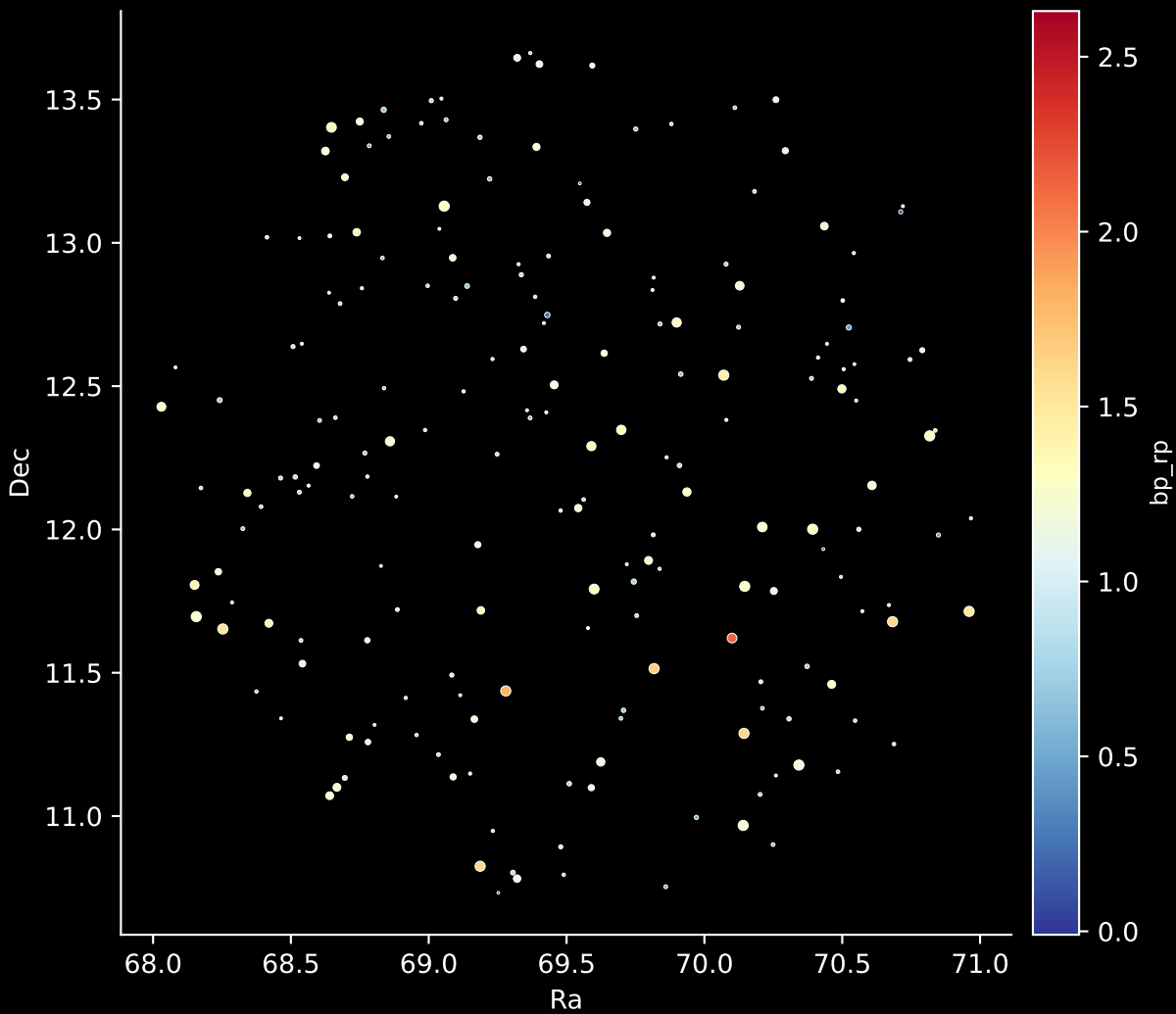
APOGEE DR17 Field: [070-32_MGA] Stars: 196
