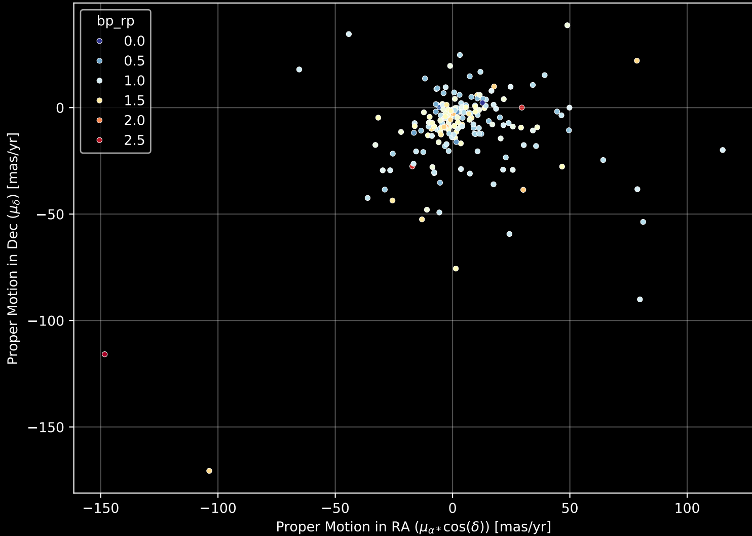
APOGEE DR17 Field: [070-32_MGA] Proper Motion Diagram (n= 196)
