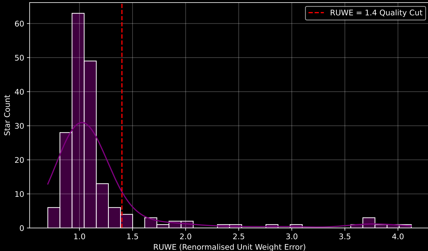
GAPOGEE DR17 Field [070-32_MGA] RUWE Distribution (n= 188)
