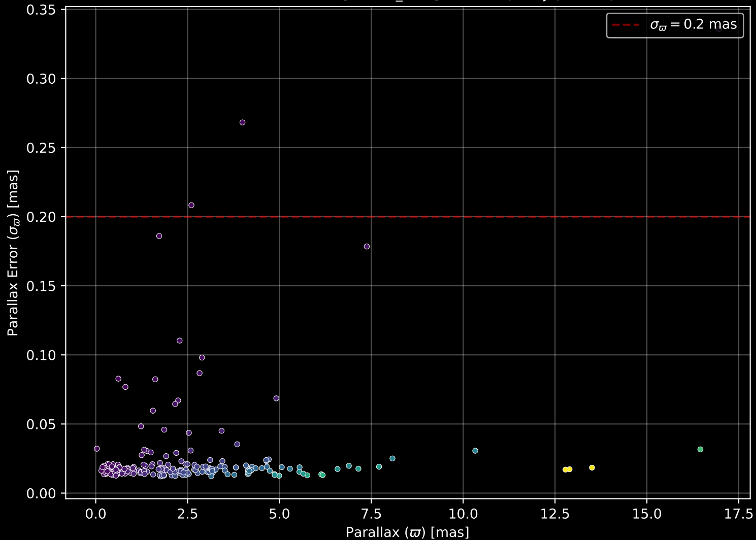
APOGEE DR17 Field: [070-32_MGA] Parallax Quality (n= 196)
