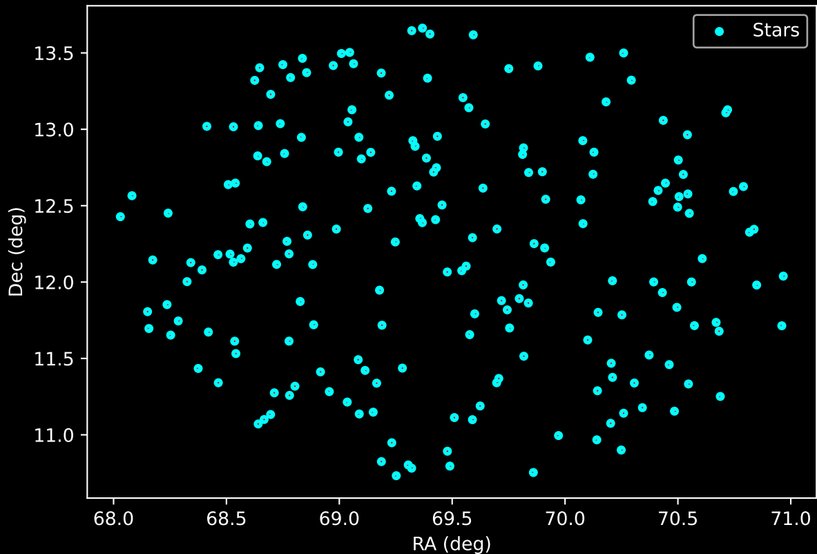
APOGEE DR17 Field: [070-32_MGA] Proper Motion Vectors for Gaia Star Field (n= 196)
